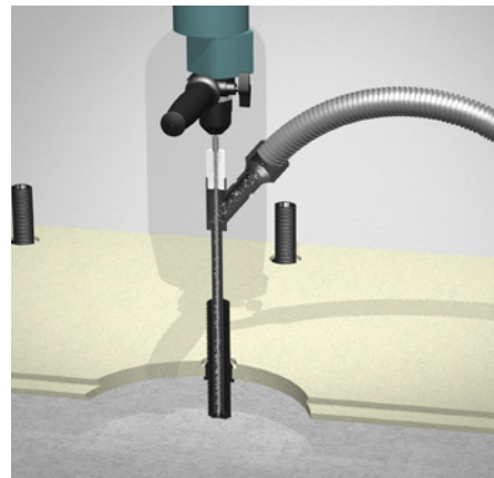
Spikexpander
